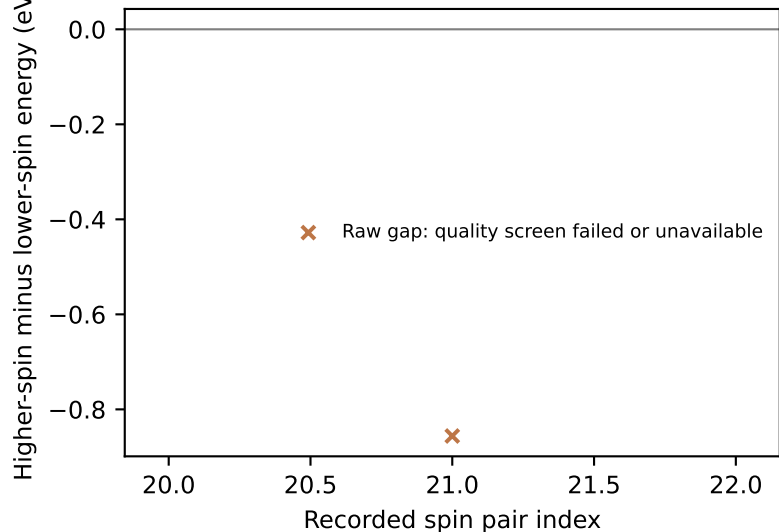
Small-basis gas-phase raw vertical gaps
