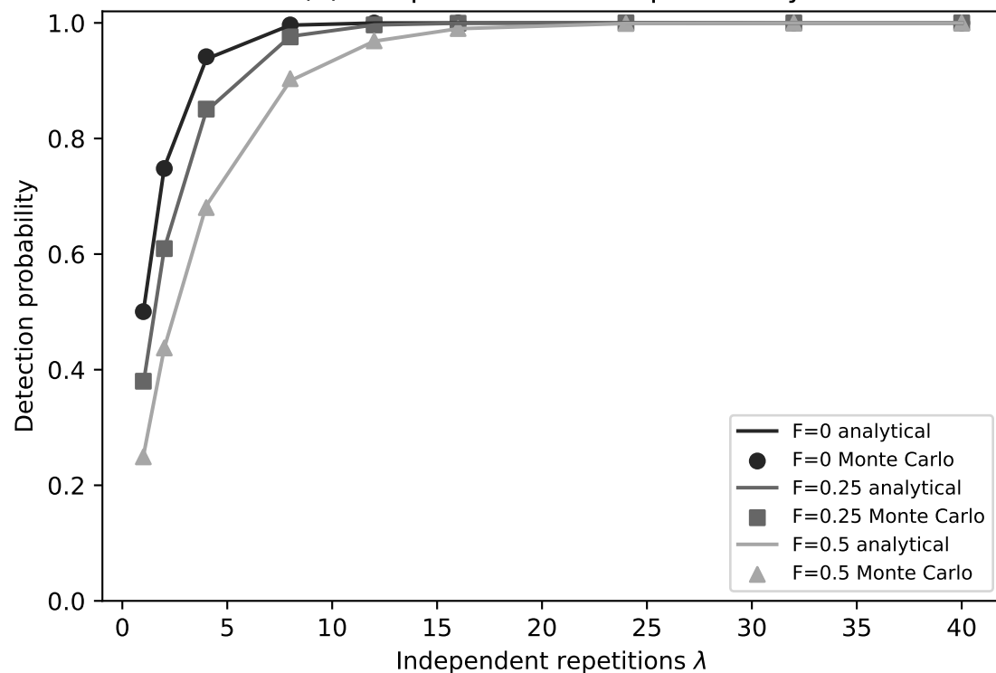
(a) Swap-test detection probability
