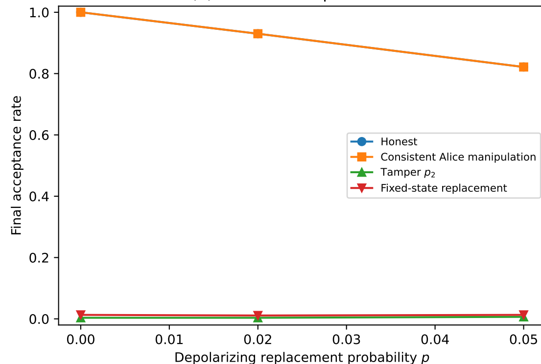
(b) Protocol acceptance rate
