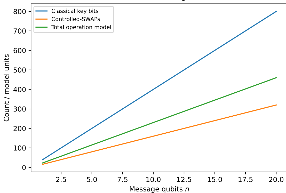
(c) Resource scaling ( \lambda = 8 )
