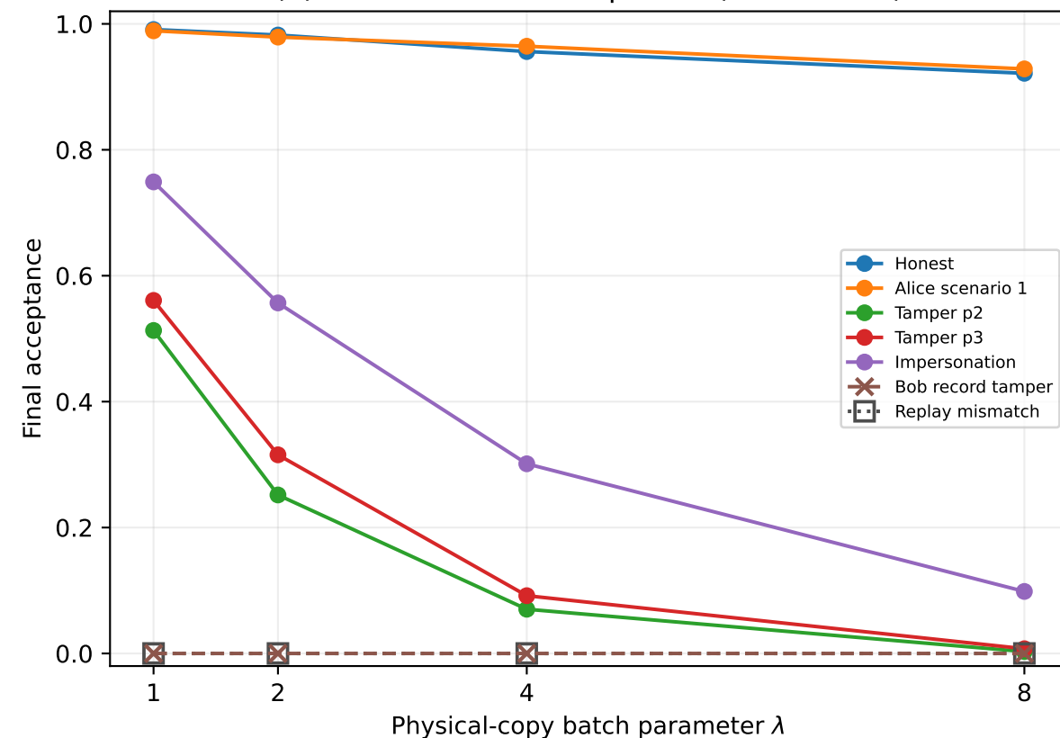
(b) Protocol-batch acceptance (noise=0.02)
