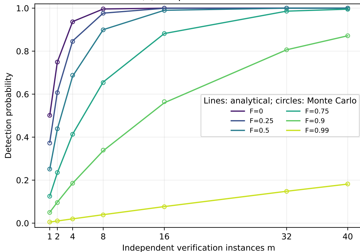
(a) Swap-test detection
