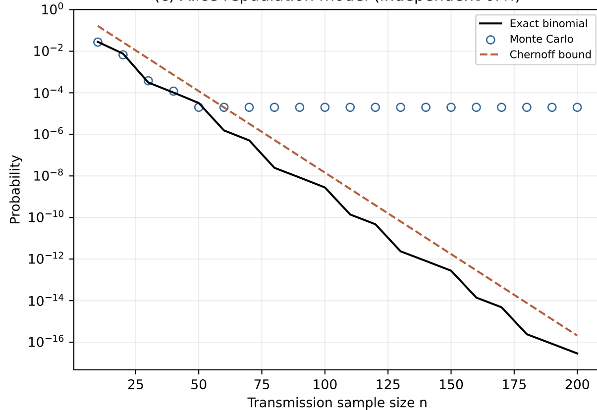
(c) Alice repudiation model (independent of \lambda )
