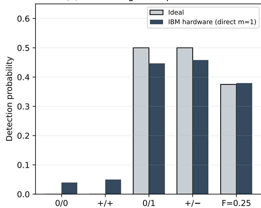
(c) Direct single Swap-Test circuits
