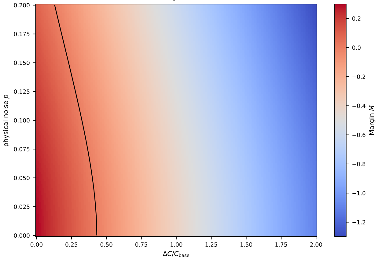
Resource margin for [[7, 1, 3]]
