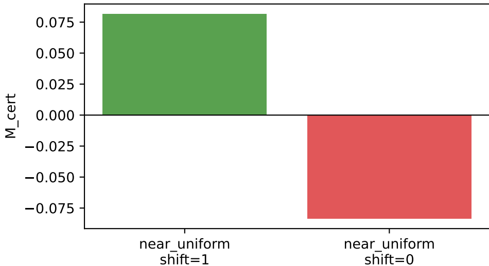
Exact SDP M=8 controlled probe
