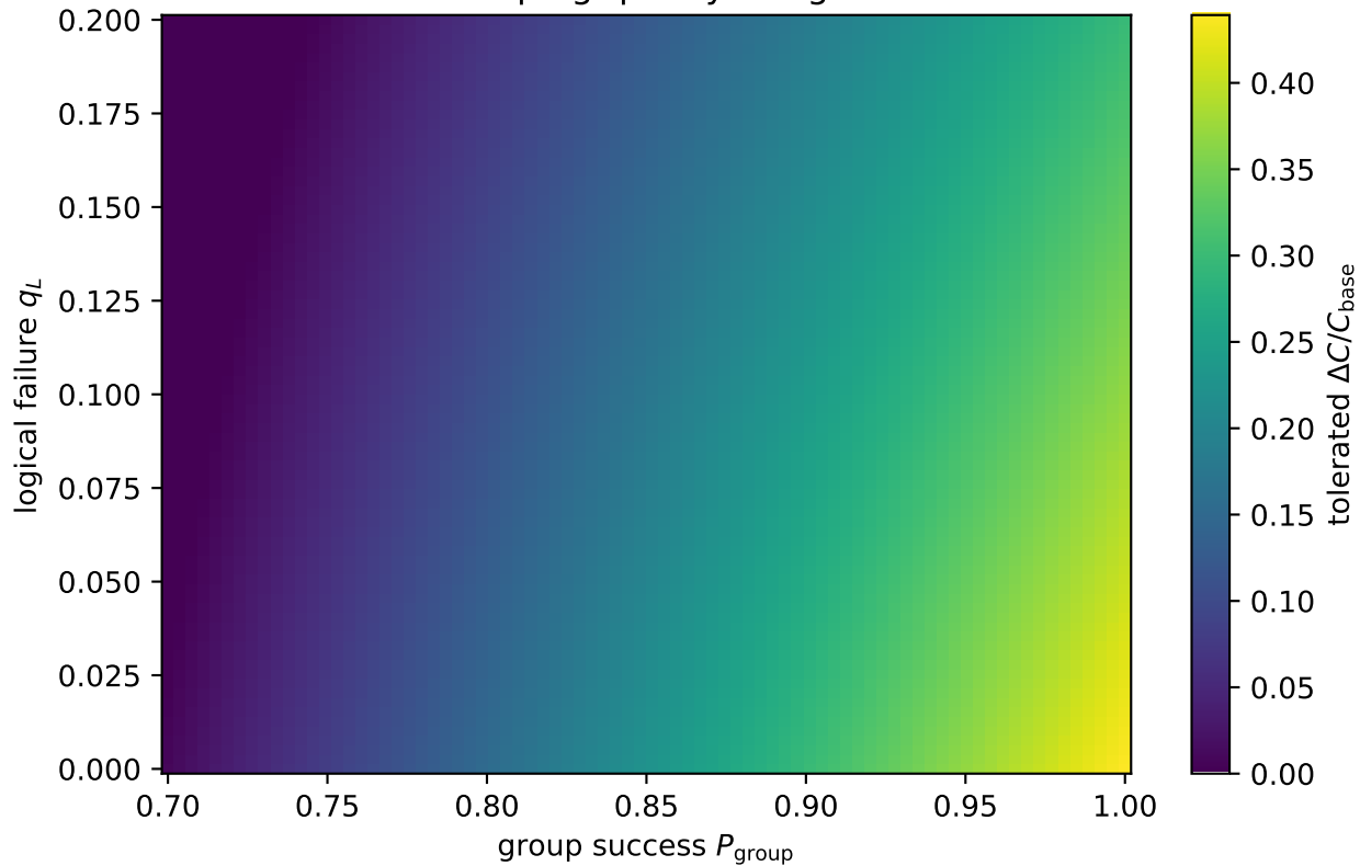
Grouping-quality margin
