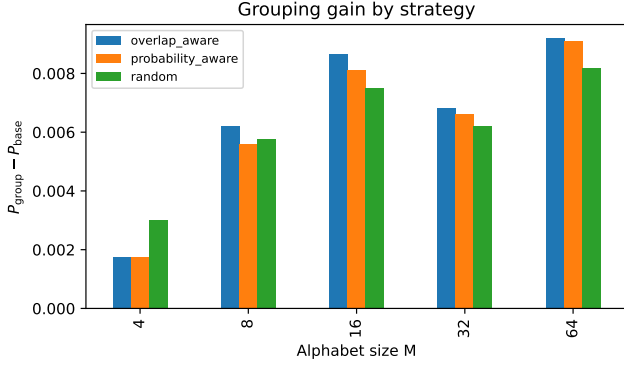
FIG. 5. Grouping gain by strategy in the multi- M benchmark. Random, probability-aware, and overlap-aware partitions are tested with fixed seeds.
