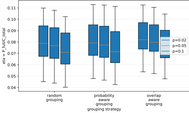
FIG. G7. Distribution of resource-normalized efficiency over randomized ensembles, using \eta = P_{\text{full}}/C_{\text{total}} with C_{\text{total}} = \bar{L} + C_A + C_{\text{QEC}} .
