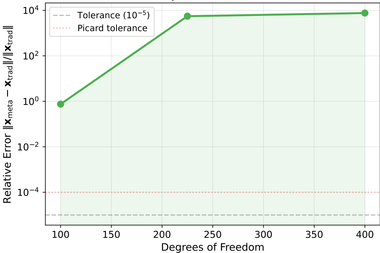
Solution Accuracy: Meta-AMG vs Traditional AMG
