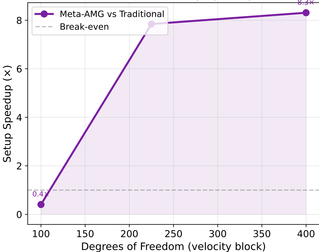
(a) Meta-AMG Setup Speedup
