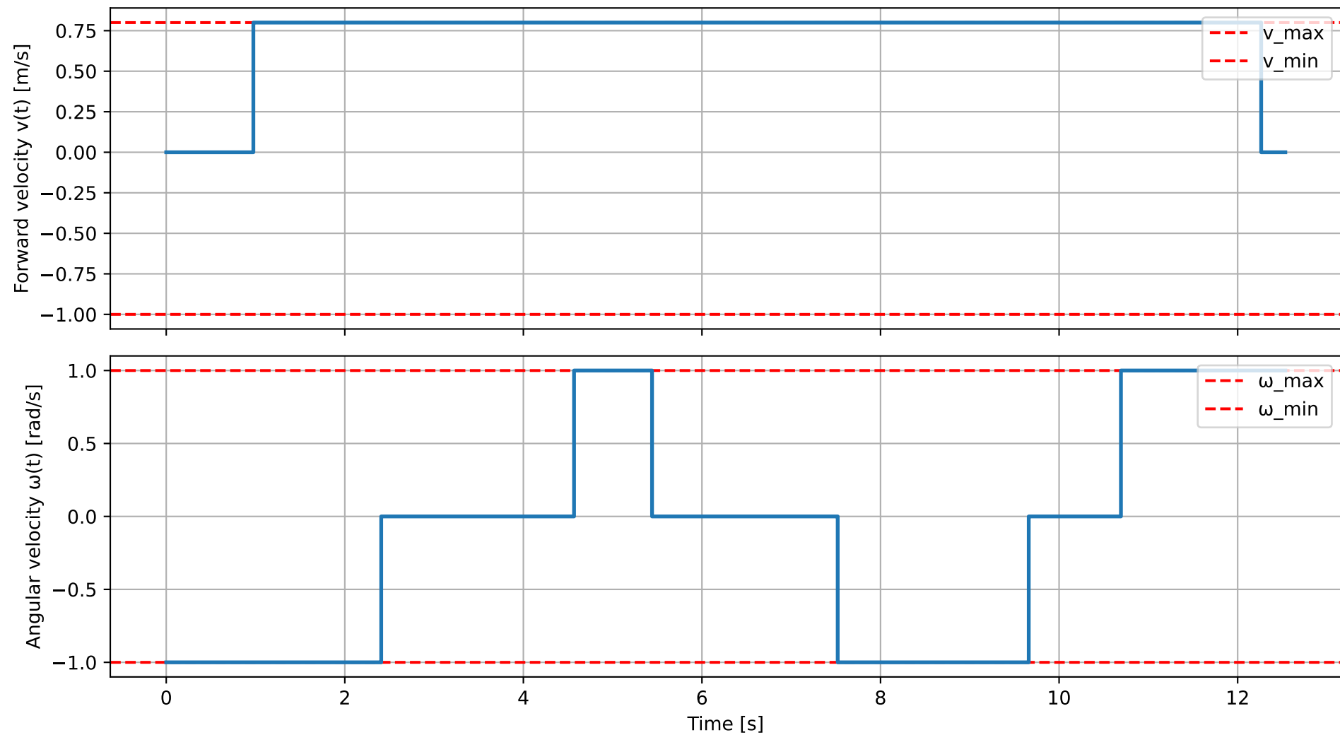
Control Profiles — Total motion time: 12.53 s
