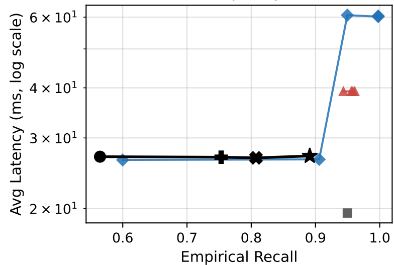
5% sparsity
