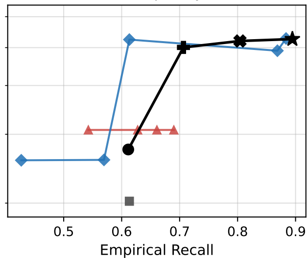
40% sparsity
