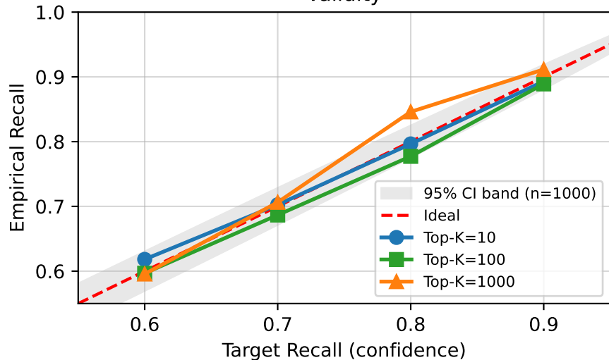
Validity
