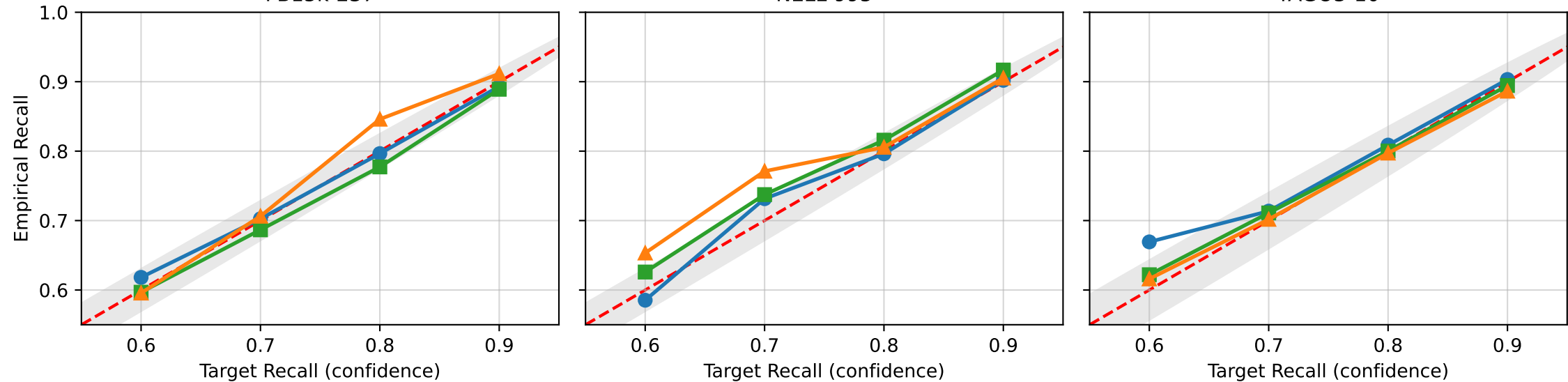
FB15k-237
