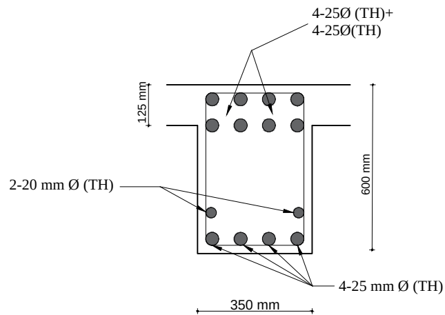
BEAM (B1) AT SUPPORT at section 29-29
