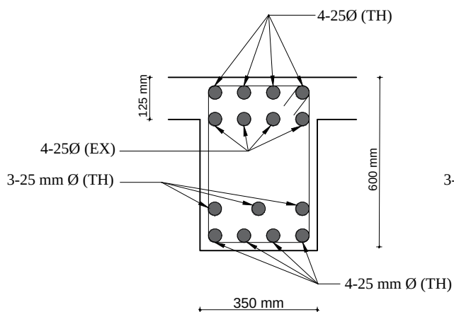
BEAM (B1) AT SUPPORT at section 25-25
