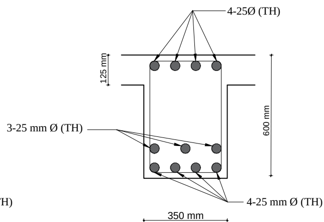
BEAM (B1) AT MID SPAN at section 26-26
