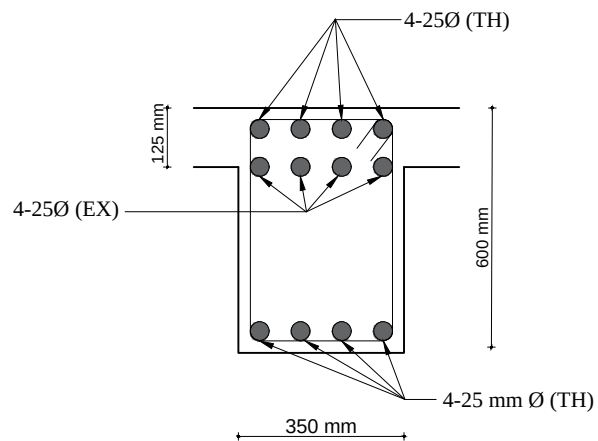
BEAM (B1) AT SUPPORT at section 38-38
