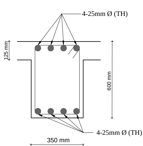
BEAM (B1) at section 5-5 AT MID SPAN
