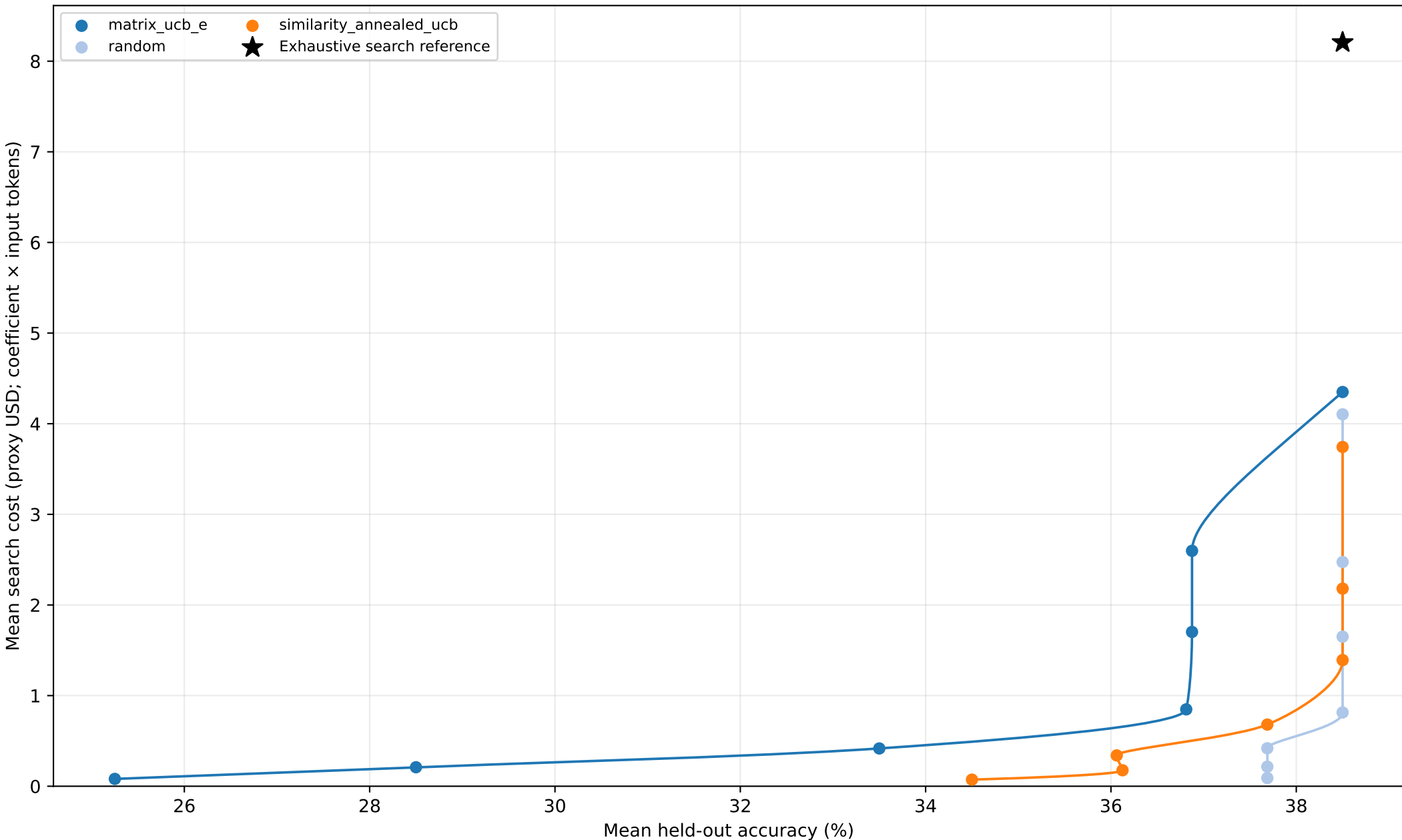
Gold-labeled offline profiling: held-out accuracy versus search cost
