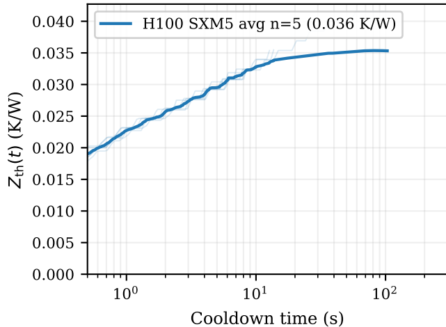
Transient thermal impedance Z_{th}(t)
