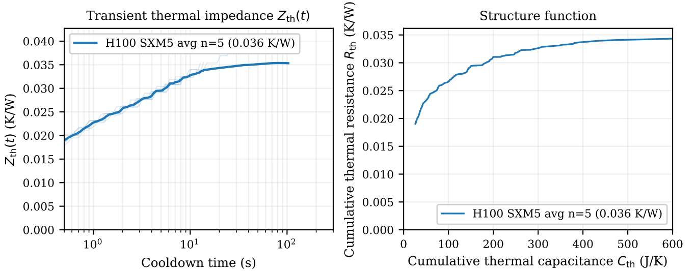
Fig. 1. Left: transient thermal impedance Z_{th}(t) for the Schmidt Sciences H100 SXM5, averaged over n=5 independent runs (bold) with individual runs shown faintly; averaging over runs reduces the effective 1^\circ\text{C} quantization noise by \sqrt{n} . Right: cumulative structure function in resistance-capacitance space, derived via R(t) = Z_{th}(t) , C(t) = t/Z_{th}(t) , and plotted to 600 J/K (the curve extends further as the liquid-cooling loop charges). The steep segment at C \lesssim 100 \text{ J/K} represents the low-capacitance, high-resistance die and package layers; the shallower rightward extension is the large-mass direct-liquid cooling path. A GPU with increased package-level thermal resistance would show a taller steep segment, lifting the entire curve and increasing Z_{th,max} .
