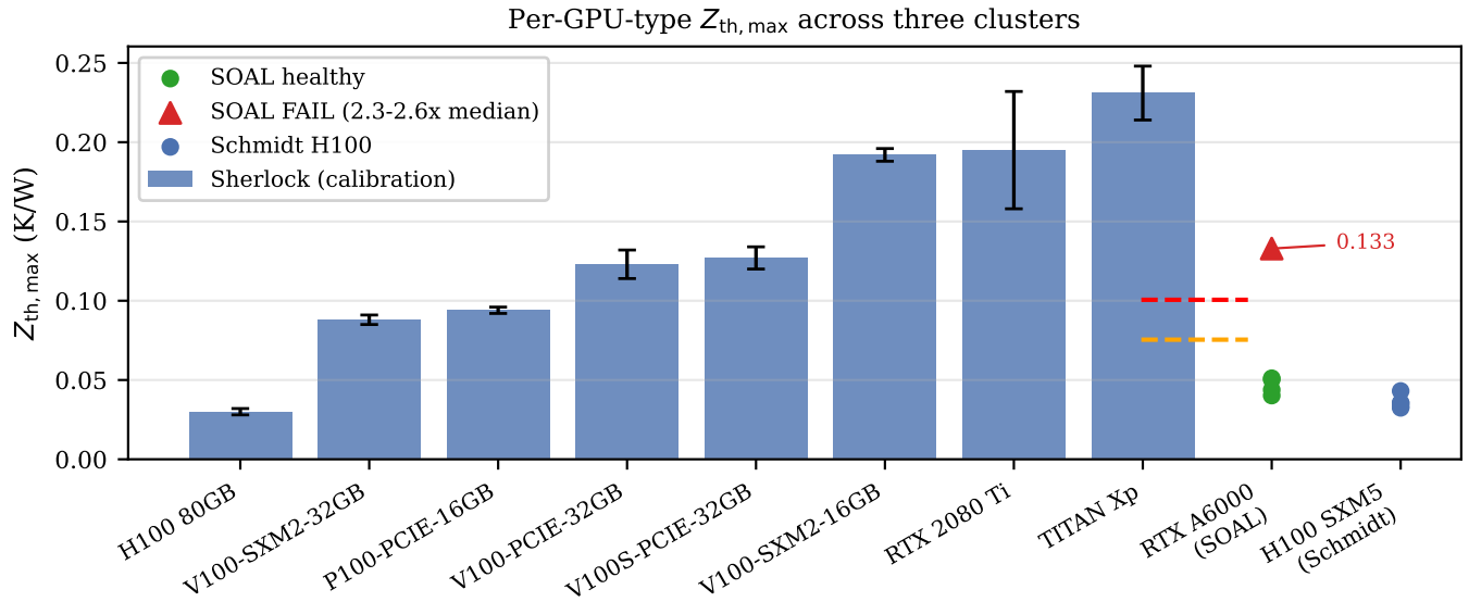
Fig. 3. Cross-cluster Z_{th,max} comparison. Bars show Sherlock per-type medians \pm\sigma (blue). Scatter points show SOAL RTX A6000 measurements (circles = healthy, triangles = FAIL) and Schmidt Sciences H100 SXM5 measurements. Dashed lines mark the WARN (1.5 \times ) and FAIL (2.0 \times ) thresholds for the A6000 type; the two annotated points exceeded the median by 2.35 \times and 2.58 \times . Schmidt H100 values (right) cluster tightly near 0.036 K/W, consistent with the Sherlock H100 median of 0.030 K/W and confirming cross-cluster portability.
