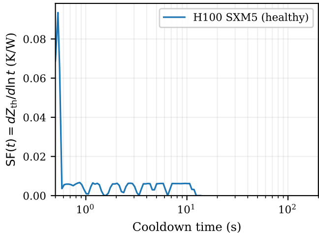
Differential structure function
