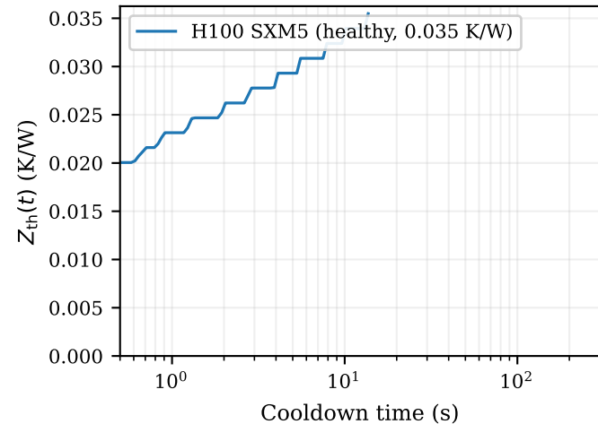
Transient thermal impedance Z_{th}(t)
