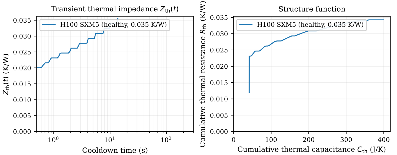
Fig. 1. Transient thermal impedance Z_{th}(t) (left) and the corresponding cumulative structure function in resistance–capacitance space (right) for the Schmidt Sciences H100 SXM5. The structure function is derived from the parametric mapping R(t) = Z_{th}(t) , C(t) = t/Z_{th}(t) , which traces the heat-flow path from die to ambient as cumulative thermal resistance (K/W) and cumulative thermal capacitance (J/K). The steep near-vertical segment at low C ( \lesssim 50 J/K) represents the low-capacitance, high-resistance die and TIM layers; the shallower rightward extension ( C \sim 100 – 400 J/K) represents the large-mass liquid-cooling loop. A GPU with degraded TIM would show a taller steep segment, shifting the entire curve upward and increasing Z_{th,max} .
