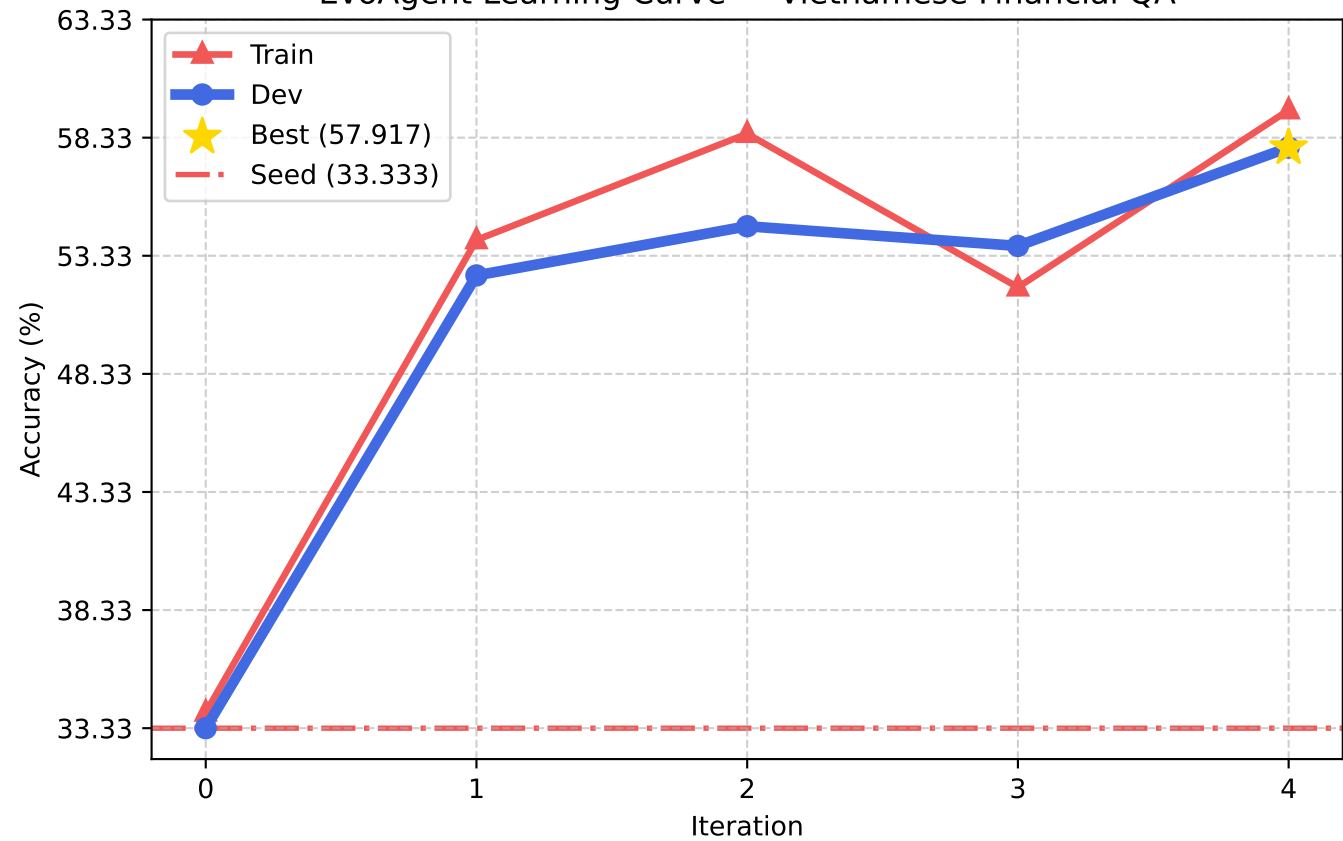
EvoAgent Learning Curve — Vietnamese Financial QA
