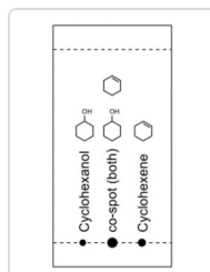
Part 2 TLC (3 lanes)
