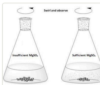
ion is dry (i.e. has no water remaining), not all of th drying w/ \text{MgSO}_4 (dry = "snow-globe")
