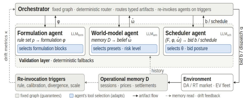
AgentV2G architecture: three role agents on a fixed graph
