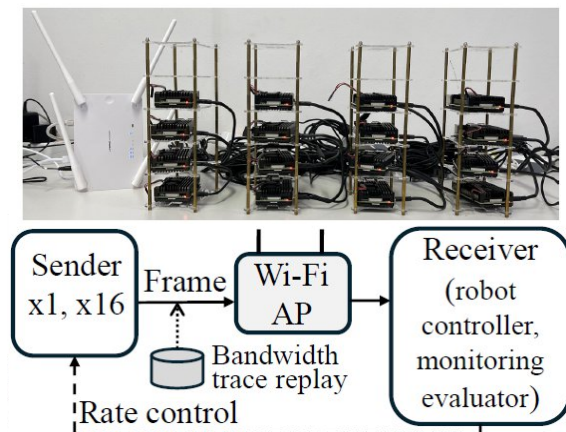
16-node Raspberry Pi 802.11ac NiL testbed
