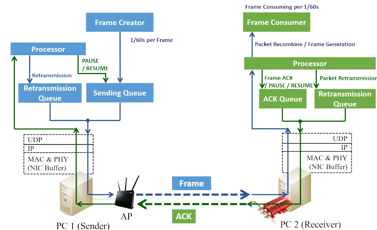
One Connect wireless streaming testbed
