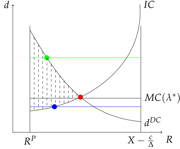
Figure 3: Oligopoly pricing
