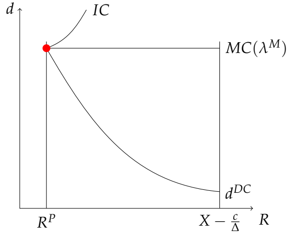
Figure 2: Monopoly pricing
