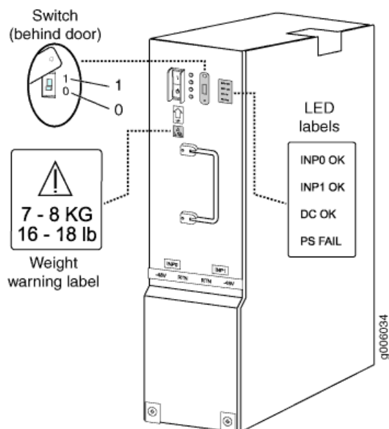
Figure 29: MX960 DC High-Capacity Power Supply Front View
