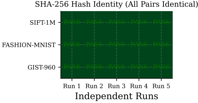
Fig. 8: Determinism verification heatmap. Each cell represents the hash comparison between two runs. Green indicates identical hashes (PASS). All cells are green, confirming perfect bit-exact reproducibility.
