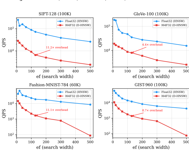
Fig. 6: Raw I64F32 search overhead (without optimizations) across four datasets. The overhead ranges from 4.4× (GloVe-100) to 11.2× (SIFT-128), demonstrating the necessity of the optimization suite.
