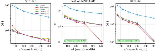
Fig. 1: Two-phase search comparison on SIFT-128, Fashion-MNIST-784, and GIST-960. The two-phase variants (with different expansion factors 2\times , 3\times , 5\times ) achieve \sim 1.08\times speedup over pure I64F32, narrowing the gap to floating-point HNSW.
