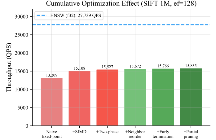
Fig. 2: Ablation study showing the cumulative effect of each optimization on SIFT-1M. Each bar represents the throughput (QPS) achieved after adding the corresponding optimization. The dashed line indicates standard HNSW throughput.
