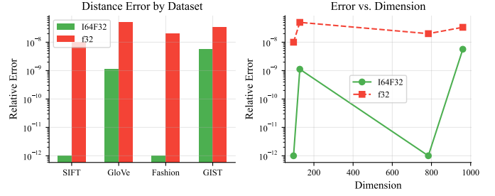
Fig. 7: Distance computation error analysis across datasets. Left: relative error distribution for i64 (fixed-point) vs. f32 (floating-point). Right: error vs. dimension, showing that i64 maintains lower error than f32 at high dimensions.
