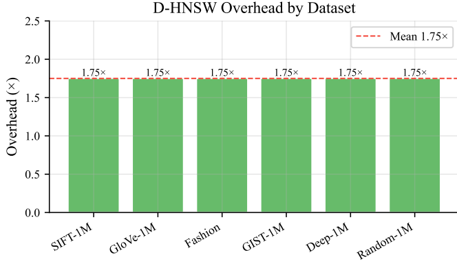
Fig. 9: Overhead breakdown across datasets. The 1.75\times overhead is consistent regardless of dimensionality, from Deep-96 (96-d) to GIST-960 (960-d).
