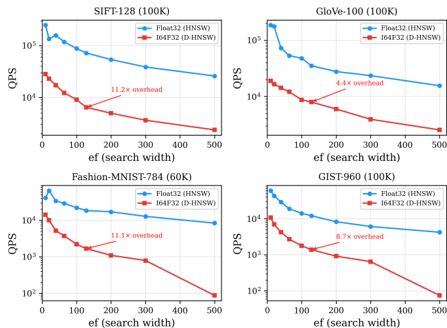
Fig. 6. Raw I64F32 search overhead (without optimizations) across four datasets. The overhead ranges from 4.4 \times (GloVe-100) to 11.2 \times (SIFT-128), demonstrating the necessity of the optimization suite.
