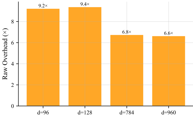
Raw I64F32 Overhead (No SIMD)
