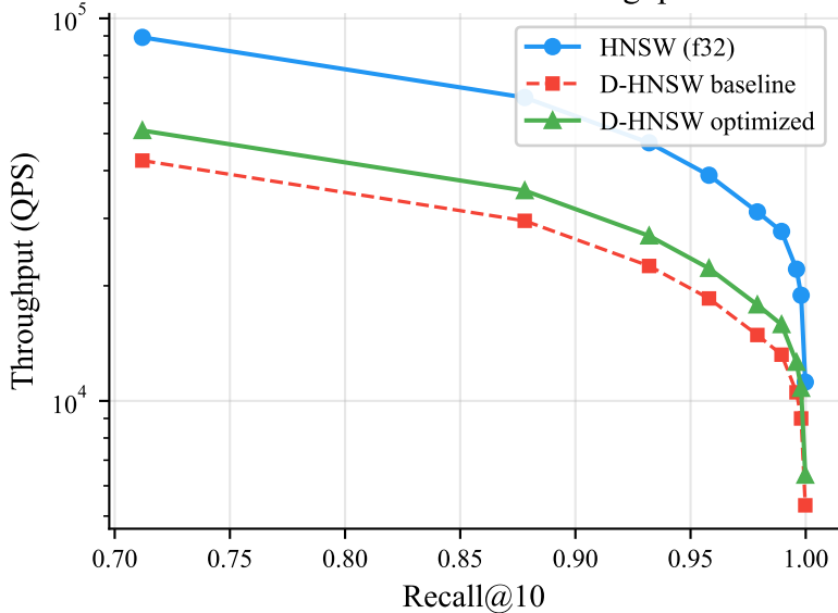
SIFT-1M: Recall vs. Throughput
