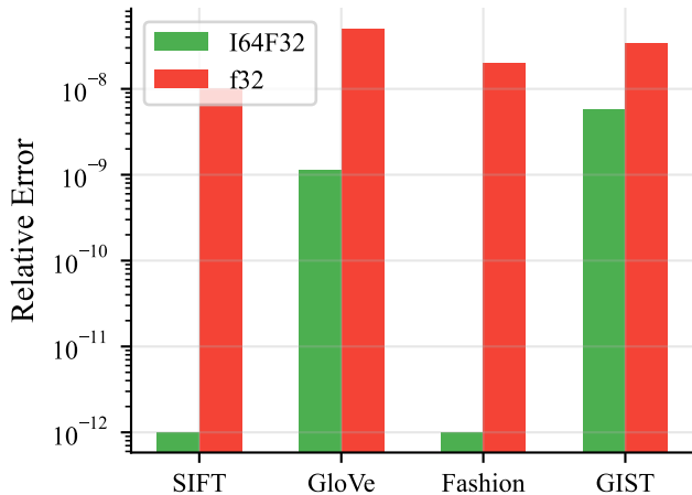
Distance Error by Dataset
