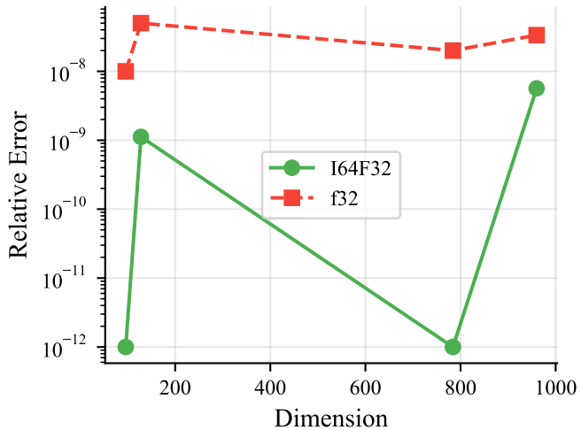
Error vs. Dimension
