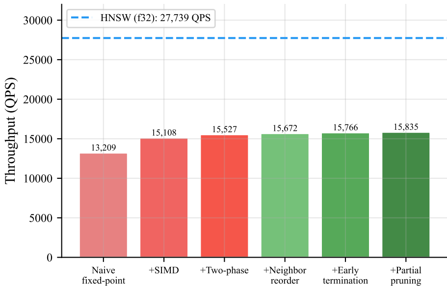
Cumulative Optimization Effect (SIFT-1M, ef=128)
