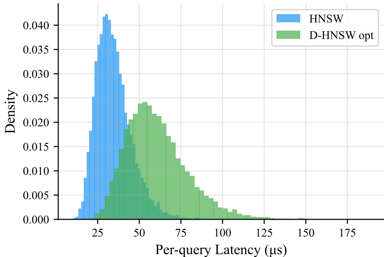
Latency Distribution (SIFT-1M, ef=128)
