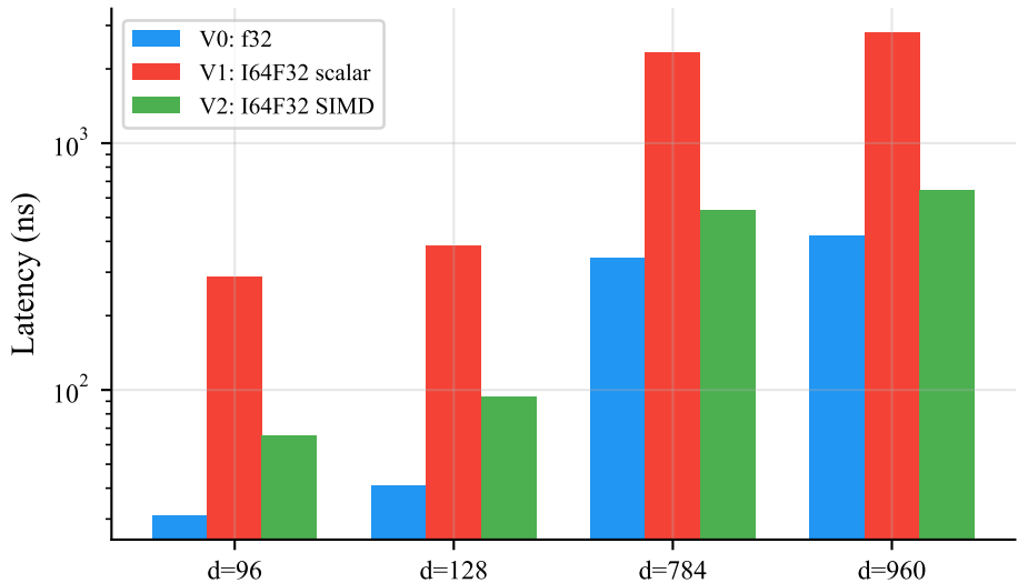
Distance Computation Latency
