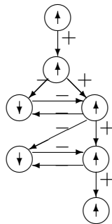
Figure 20: Consistent assignment for simple MAPK cascade model
