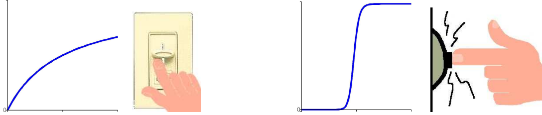
Figure 13: (a) hyperbolic response (b) sigmoidal response
