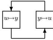
Figure 11: Feedback interconnection of two systems
