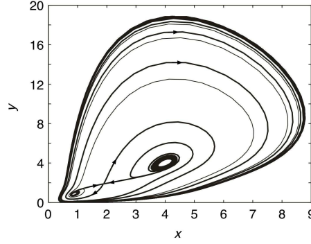
Figure 17: Phase plane for counterexample
