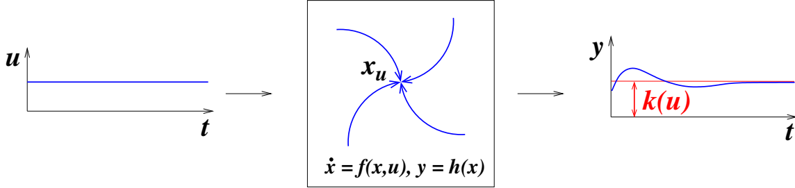
Figure 12: Characteristics: (a) constant input, (b) convergence of internal states, (c) convergence of output to value k(u)
