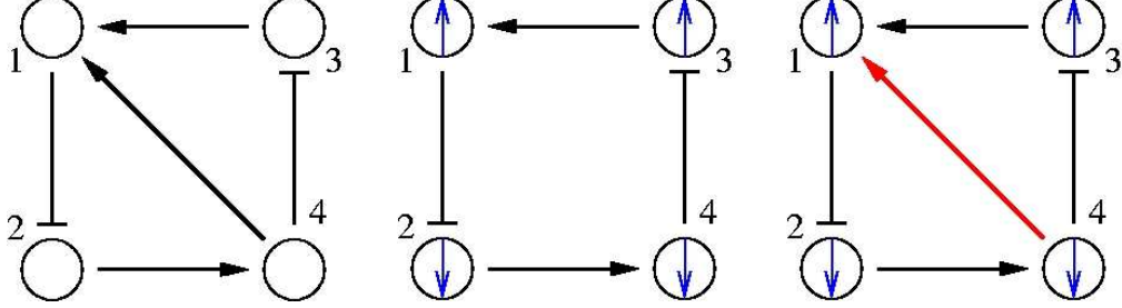
Figure 6: (a) inconsistent graph, (b) consistent subgraph, (c) one inconsistent edge
