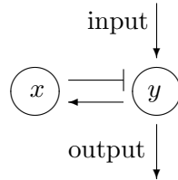
Figure 18: Influence graph for counterexample
