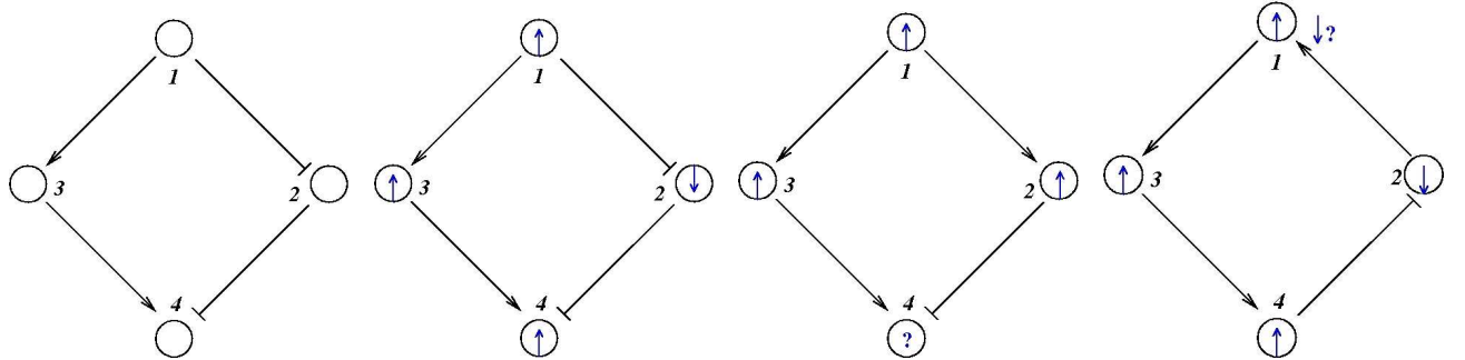
Figure 4: (a) and (b) graph and consistent assignment, (c) and (d) no possible consistent assignments
