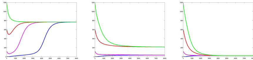
Figure 21(a),(b),(c) y_3 , g = 1/0.98, 1/2.1, 1/6
