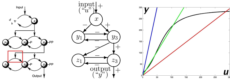
Figure 19: (a) MAPK cascades; (b) graph; (c) characteristic
