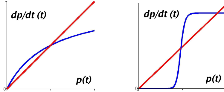
Figure 14: intersections of hyperbolic and sigmoidal response with degradation
