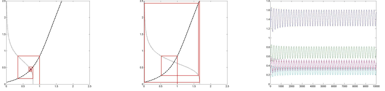
Figure 25: (a) convergent iteration; (b) divergent iteration; (c) oscillations
