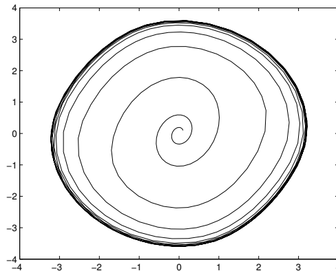
Figure 26: Limit cycle in counterexample
