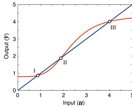
Figure 16: Characteristics for counterexample
