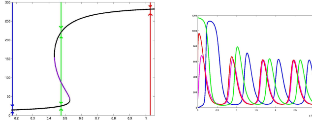
Figure 22: (a) bifurcation diagram and relaxation (b) oscillation ( y_3 )
