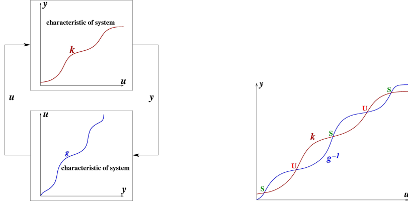
Figure 15: (a) Positive feedback
