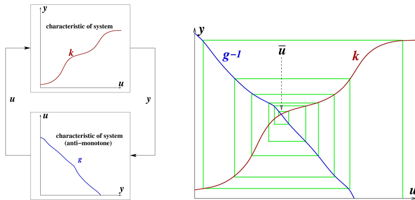
Figure 23: (a) Negative feedback and (b) characteristics
