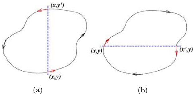
Fig. 9. Impossible (a) counterclockwise and (b) clockwise periodic orbits in planar cooperative system, each drawn in the (x, y) -plane
