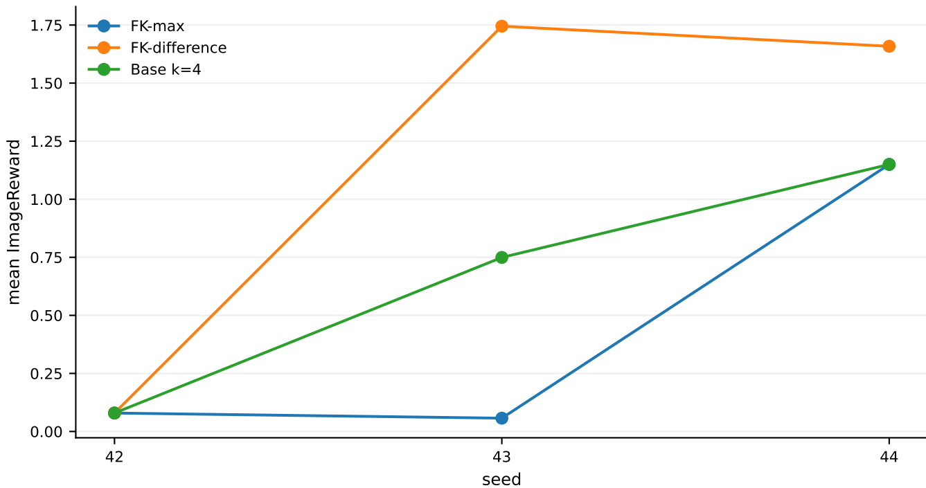
FK Steering one-prompt seed variance
