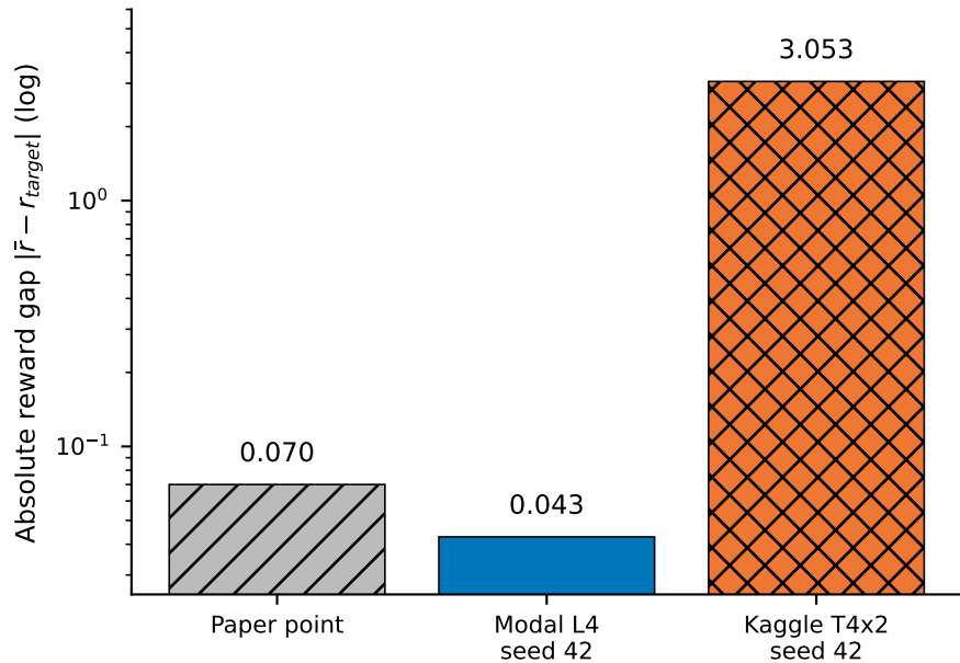
(b) Reward fidelity diagnostic
