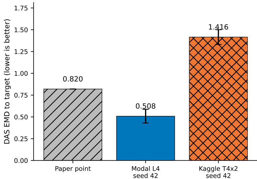
(a) Same method, same seed, different backend
