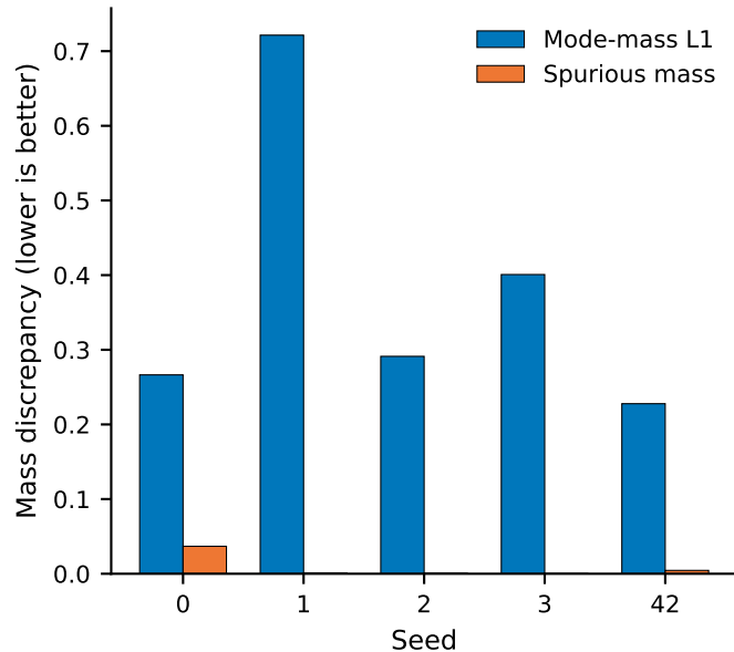
(b) Mode fidelity by seed
