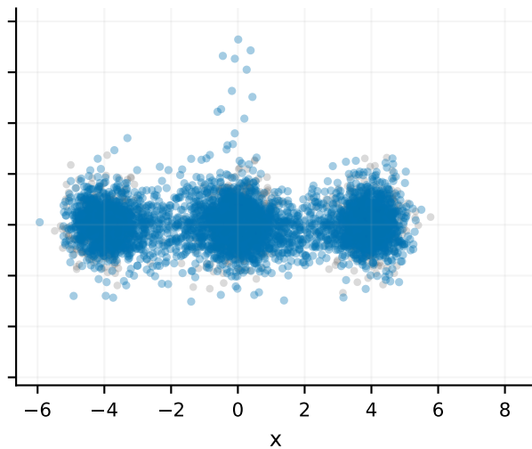
seed 44; EMD=0.505
