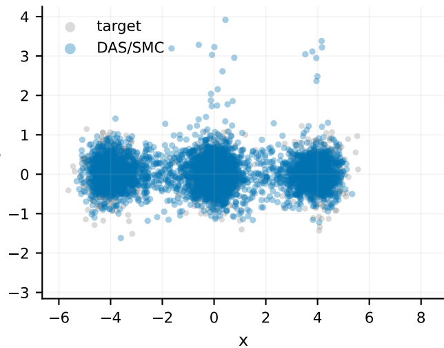
seed 42; EMD=0.743
