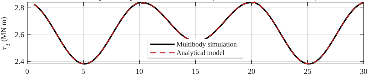
Saddle-joint torque: forward validation ( R^2 = 1.000000 , sensed accel.)
