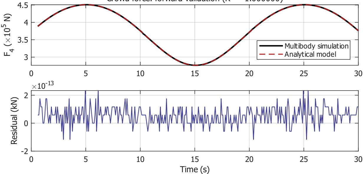
Crowd force: forward validation ( R^2 = 1.000000 )
