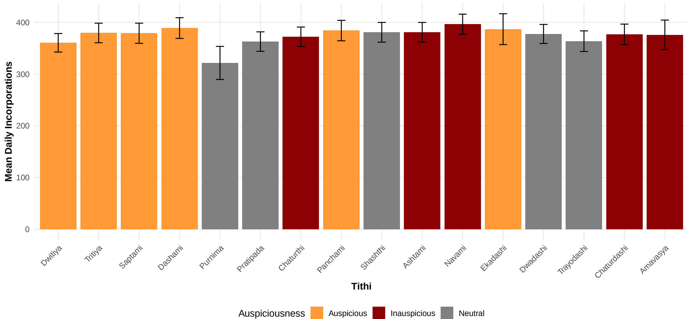
Mean Daily Incorporations by Tithi
