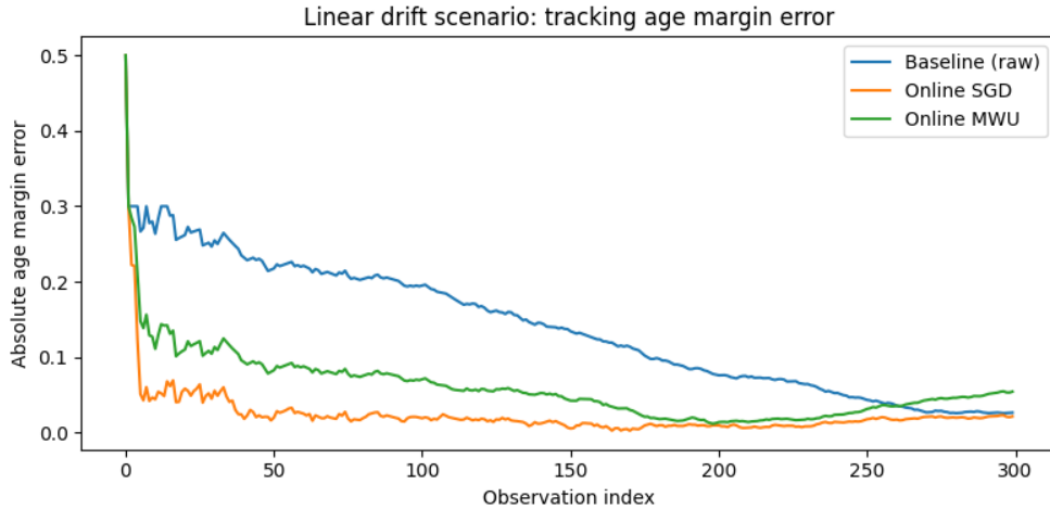
Figure 1. Absolute age margin error over time in the linear drift scenario (mean over five seeds). Online rakers quickly track the target margin, whereas the unweighted baseline drifts with the sampling bias. SGD converges slightly faster than MWU.
