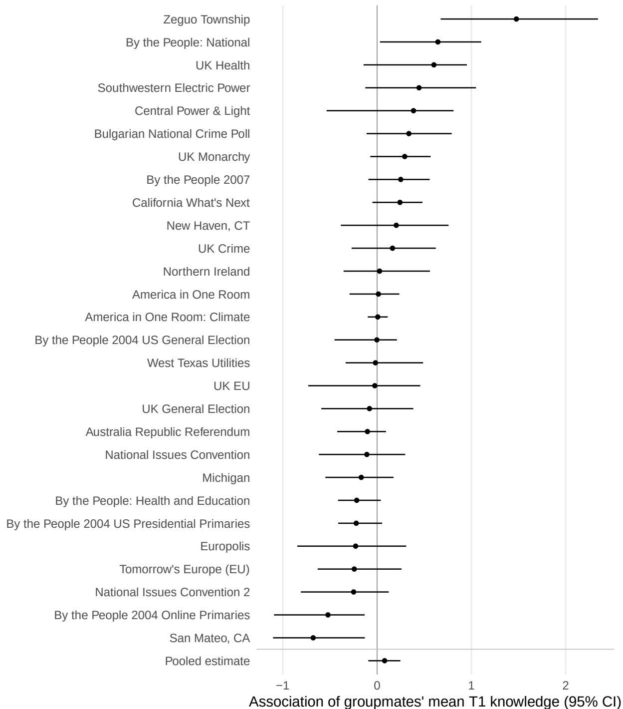
Figure B1: Association between the other group members' mean T1 knowledge and own knowledge gain, by poll, with 95% intervals. Each estimate controls for own T1 knowledge. Intervals use the hierarchical bootstrap. The pooled estimate weights polls equally and resamples polls within mode and then their groups. These are descriptive associations.
