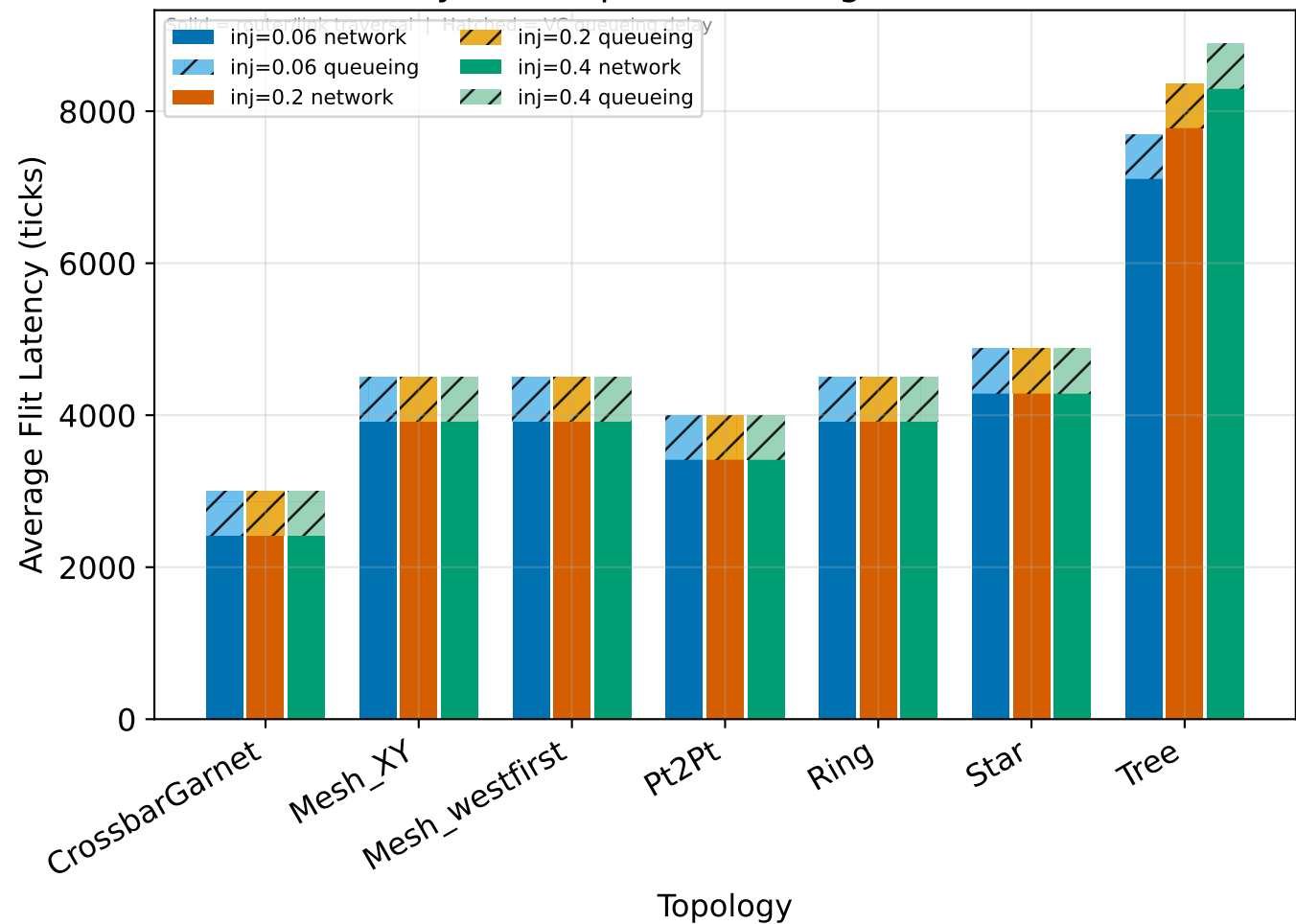
Latency Decomposition - neighbor, 16 nodes
