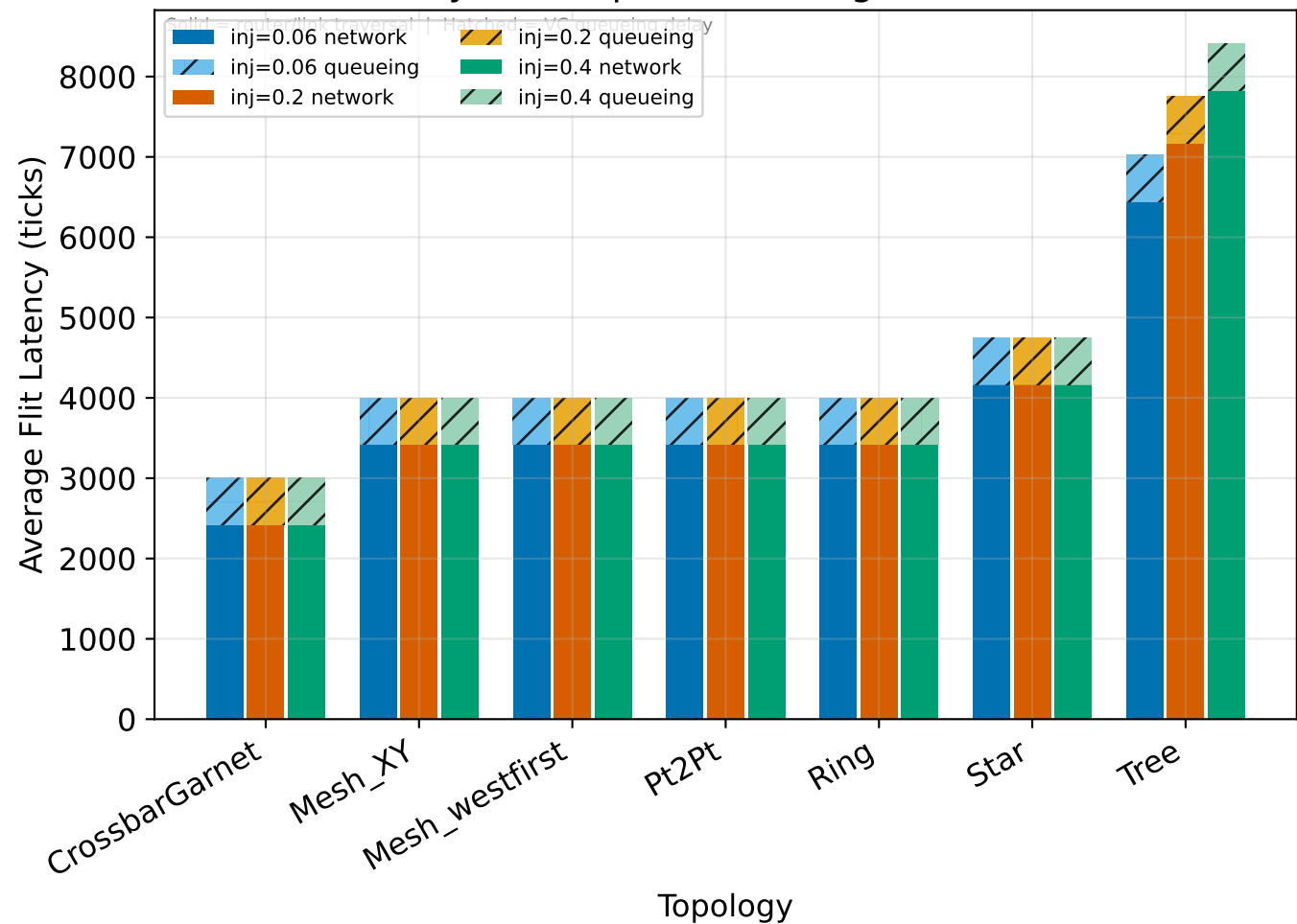
Latency Decomposition - neighbor, 8 nodes
