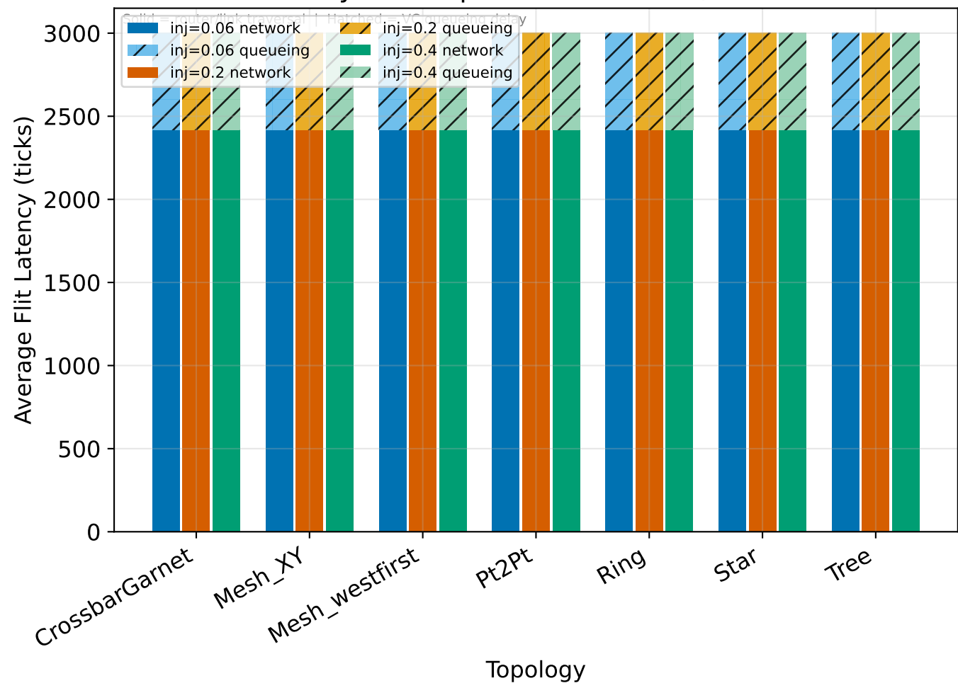
Latency Decomposition - tornado, 8 nodes
